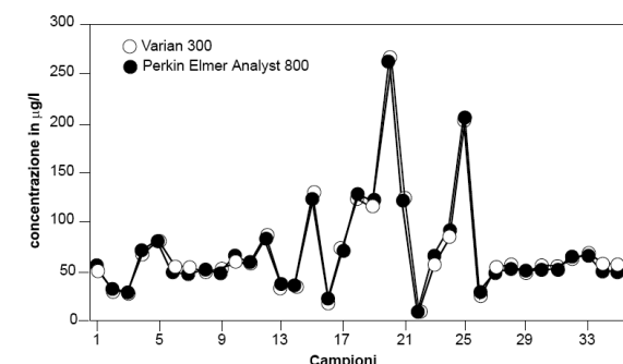
Figura 8. Confronto Varian 300/Perkin Elmer Analyst 800
